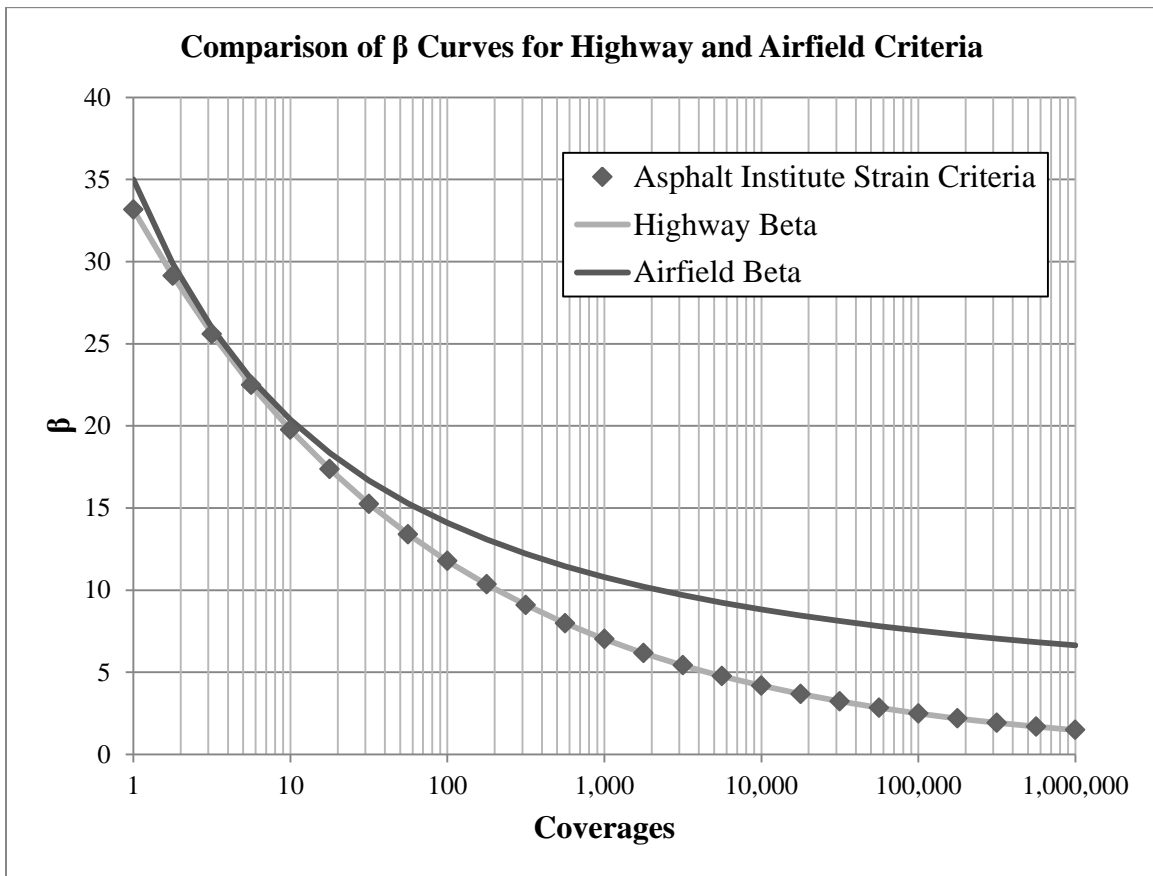
Figure 26. Comparison of \beta Curves for Highway and Airfield Criteria
