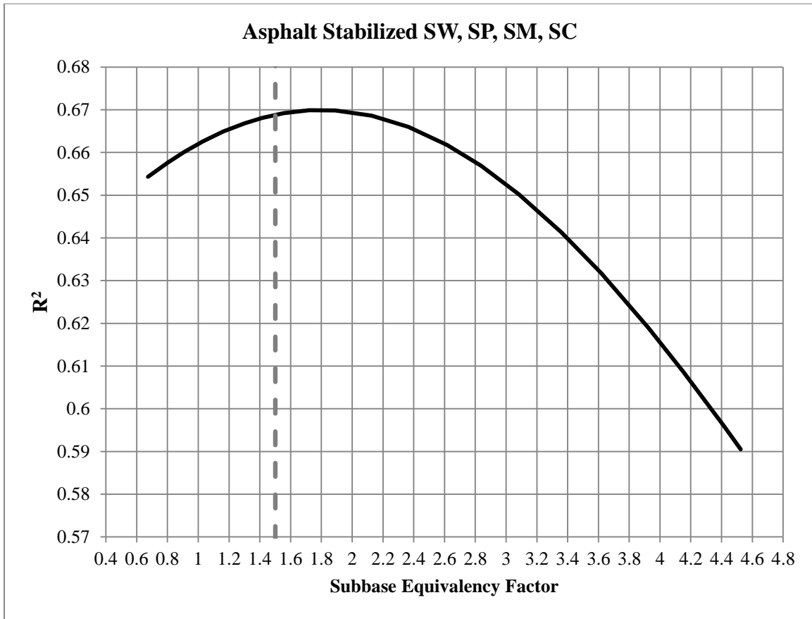
Figure 42. Optimization Curve for Asphalt-stabilized SW, SP, SM, SC Subbase Course Equivalency Factor
